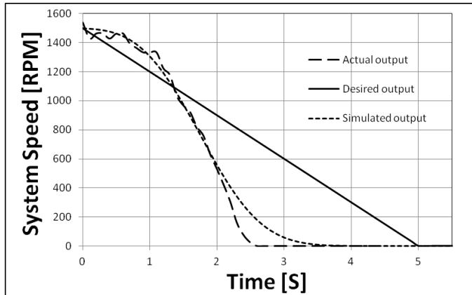
Figure.5 (Braking in 5 Sec 'open loop')
