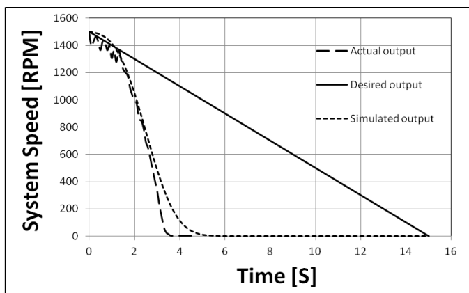
Figure.6 (Braking in 15 Sec 'open loop')
