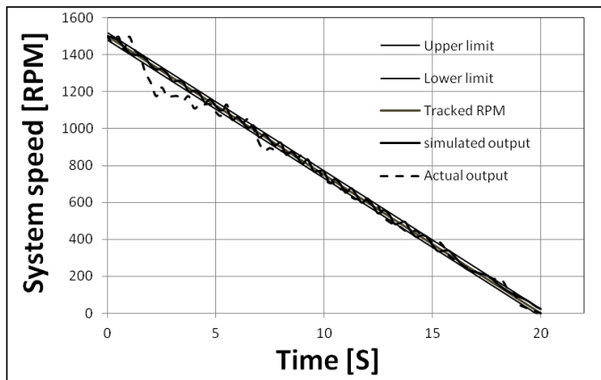
Figure.9 System response (Braking in 20 sec with a range \pm 20 RPM)
