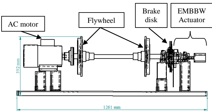
Figure.1 Mechanical laboratory setup schematic
