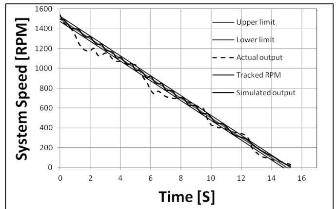
Figure.11 System response (Braking in 15 sec with a range \pm 20 RPM)
