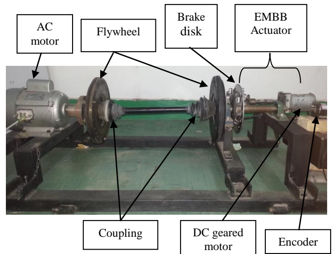
Figure.2 Mechanical laboratory setup
