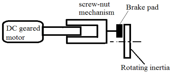
Figure.4 BBW system schematic
