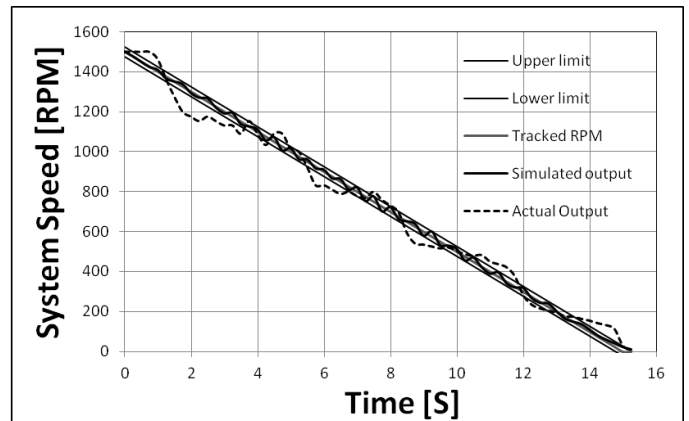
Figure.12 System response (Braking in 15 sec with a range \pm 10 RPM)
