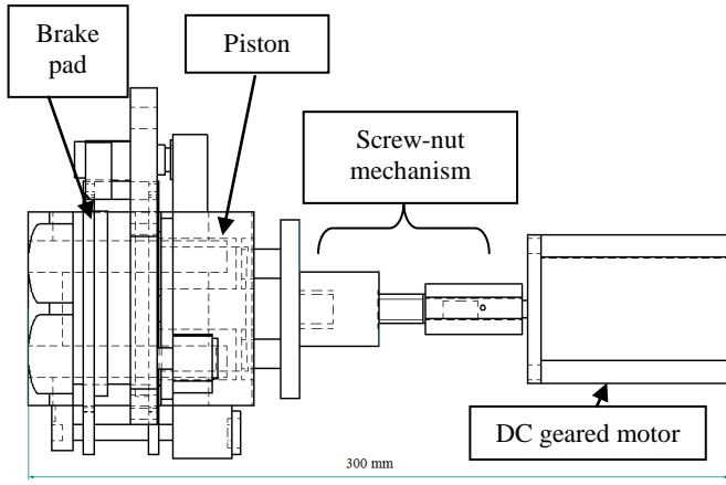
Figure.3 EMBBW Actuator
