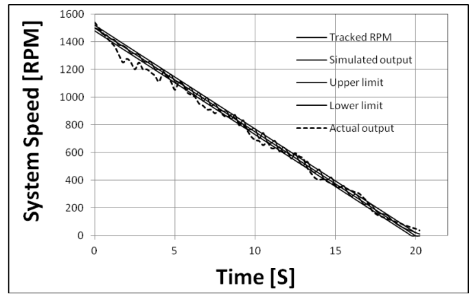
Figure.10 System response (Braking in 20 sec with a range \pm 10 RPM)
