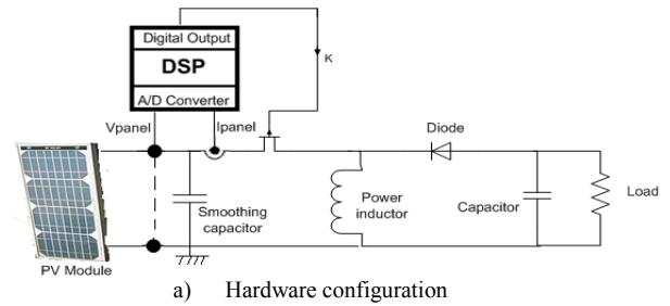
a) Hardware configuration
