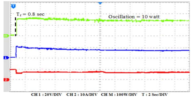
Fig 17 The Proposed Fuzzy Logic Method Practical Result
