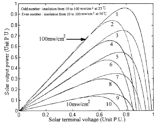
Fig. 4 The Effect of cell's temperature and solar radiation on PV Cell's P-V Curve
