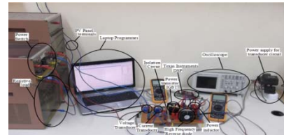
b) Photograph of setup
