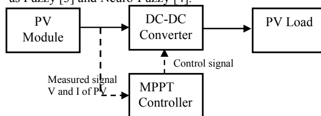
Fig. 1 PV with MPPT Configuration
