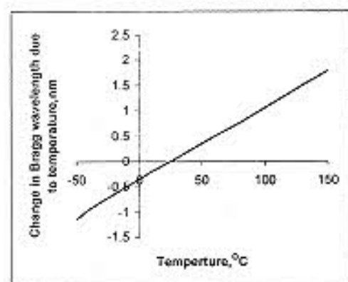
Fig. 11 The change in Bragg wavelength with temperature.
