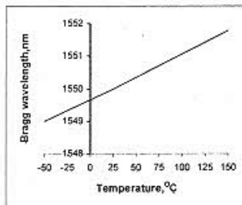
Fig.1 Bragg wavelength, \lambda_B , versus temperature.
