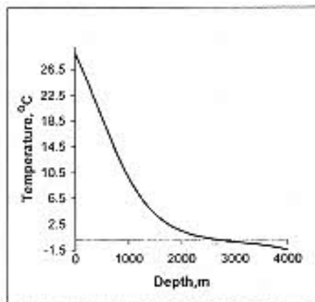
Fig. 5 Temperature versus depth.
