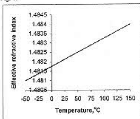
Fig. 3 FBG effective refractive index versus temperature.
