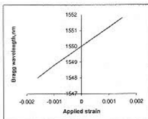
Fig. 4 Wavelength of fiber Bragg grating under applied strain.
