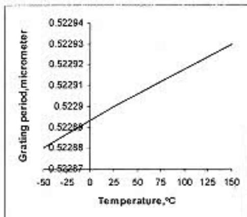
Fig. 2 Grating period versus temperature.
