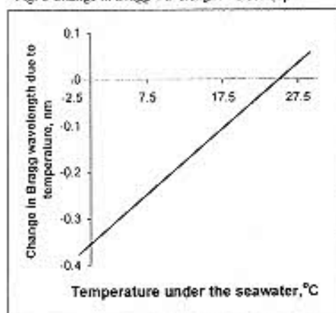
Fig. 7 Change in Bragg wavelength with temperature.
