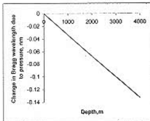
Fig. 6 Change in Bragg wavelength versus depth.
