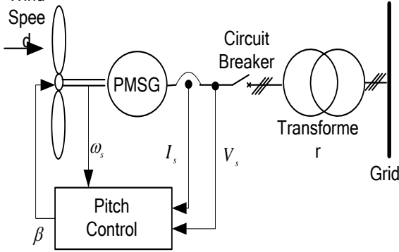
Figure 2: Control of Blade Pitch Angle
