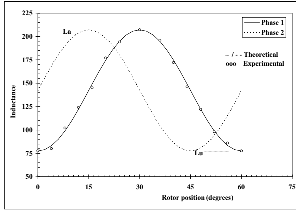
Fig.(1) The relationship between phase inductance and the rotor position
