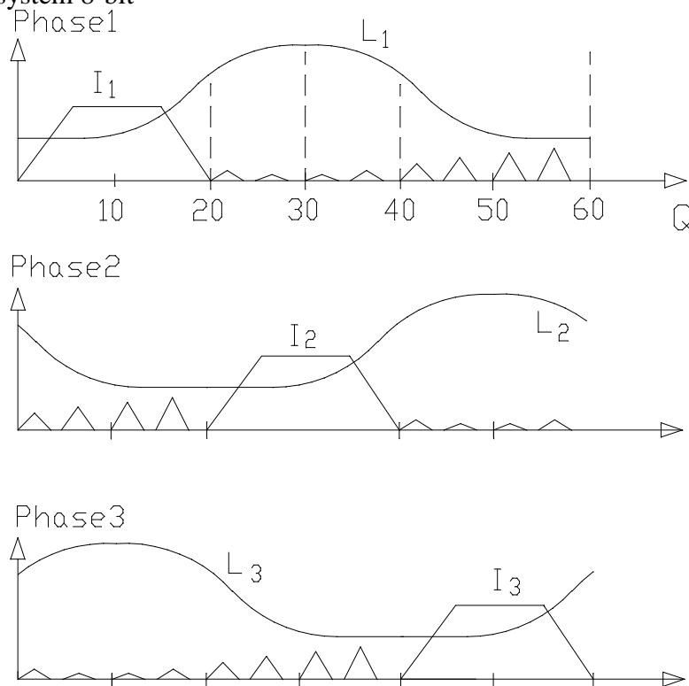
Fig. (10): Current waveforms of the 3-ph SRM
