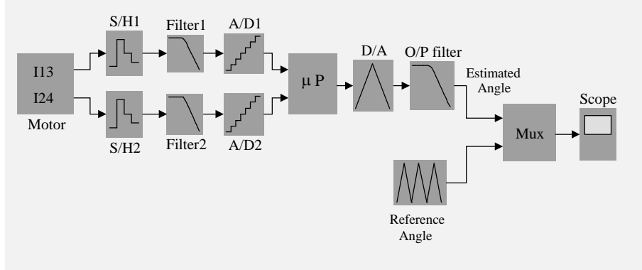
Fig. (5) Schematic diagram for the position detection circuit simulation
