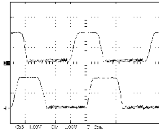
Fig. (8): Experimental current waveforms in two adjacent phases at 1000 rpm
