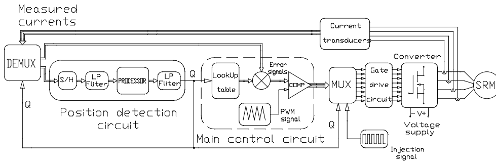
Fig(3) Schematic diagram for the drive system
