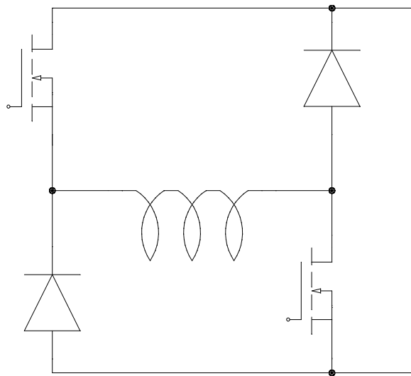
Fig. (4) Asymmetric half bridge converter per phase
