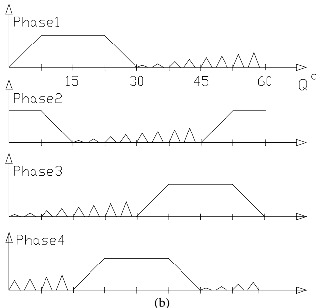
Fig. (2): (a) Inductance, voltage and current during phase injection and (b) current waveforms of the 4-ph SRM
